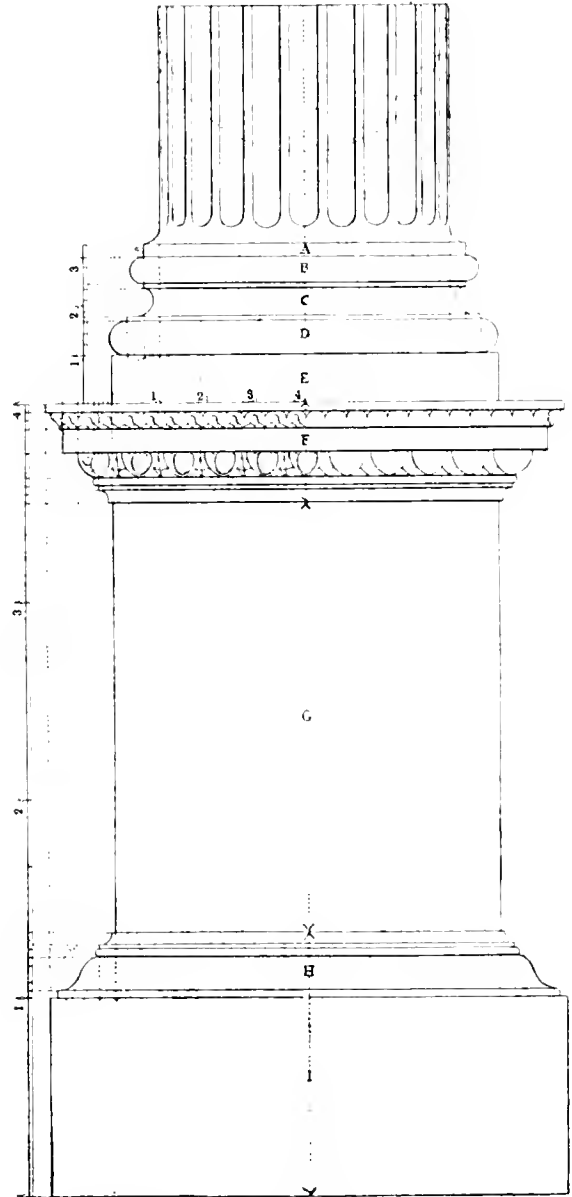
NO. 218.—SLITTING OUT AN IONIC PEDAESTAL FOR A COLUMN.
